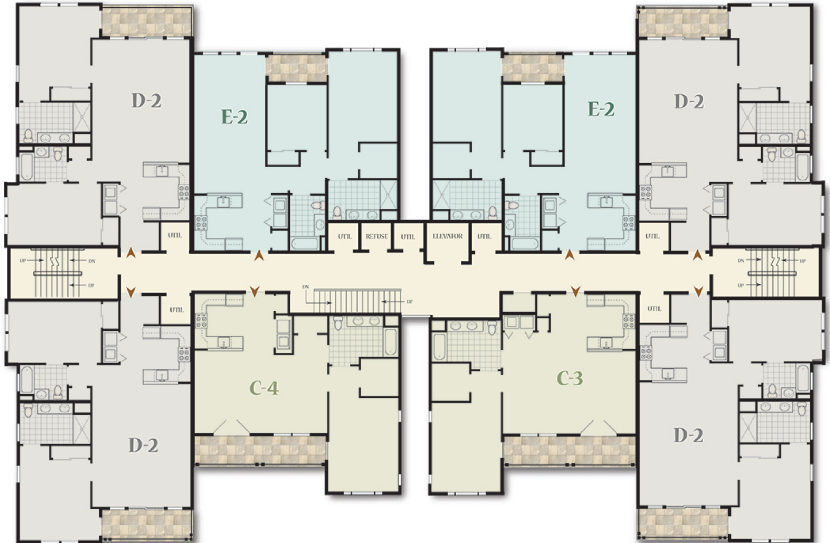
THIRD FLOOR
